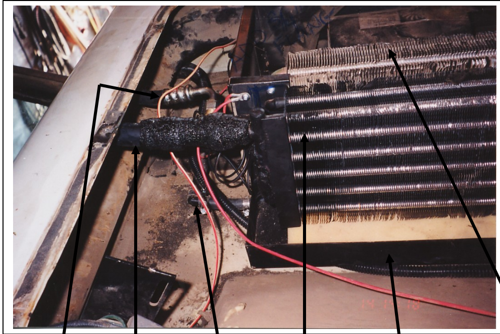
5/16" A/C hose 1/2" A/C hose Drain Hose Evaporator Coil Drain Pan Factory Heater
